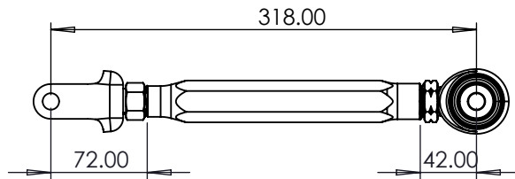
MIN ADJUSTMENT
