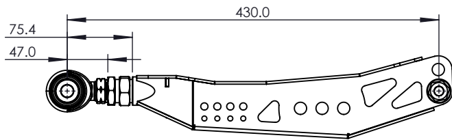
OEM LENGTH - 430MM
