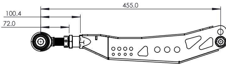
MAX LENGTH - 455MM
