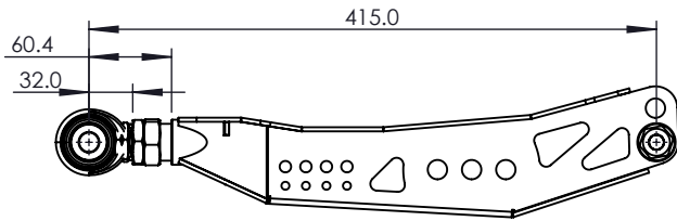
MIN LENGTH - 415MM
