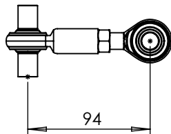
OEM/MAX ADJUSTMENT
