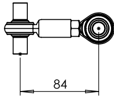
MIN ADJUSTMENT
